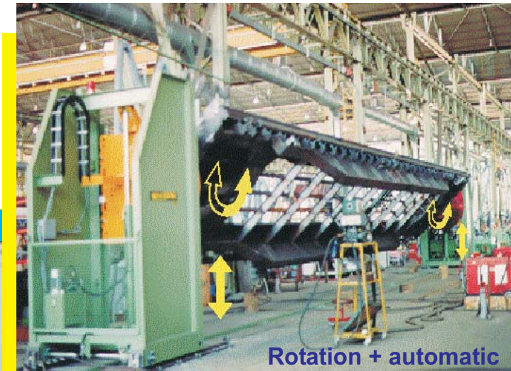
WELDING BOGIES 2 Rotations + automatic self aligning Hydraulic Lifting
